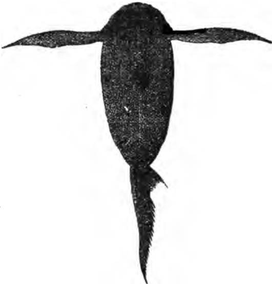
PTERICHTHYS OBLONGUS. One-half nat. size.
